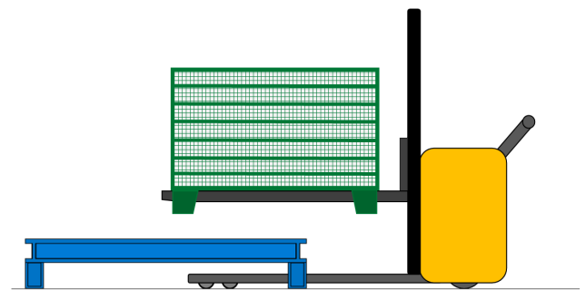
Floor scale in protective frame, accessible for lifting equipment
